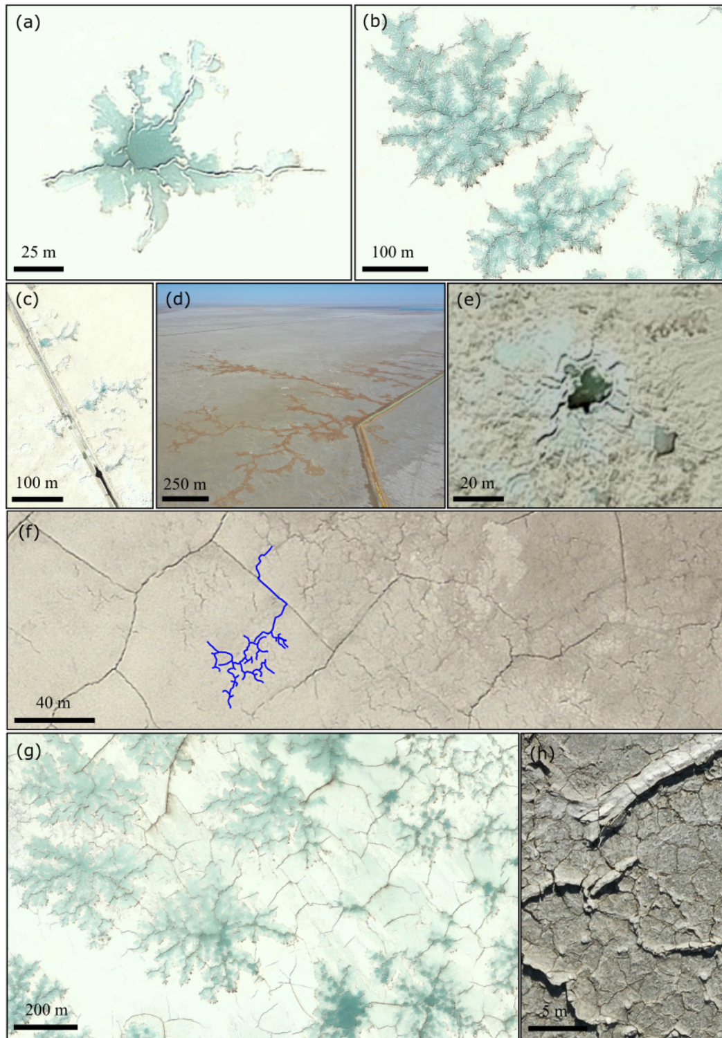
Fig. 4. The Qaidam spiders with different morphologies. (a) The early stage of the Qaidam spider. (b) The middlescence stage of the Qaidam spiders. (c, d) Parallel spiders formed along artificial saltwater canals. (e) A fat spider. Figs. 4a–c & 4e are Google satellite images taken on November 28, 2012. Fig. 4d is the aerial image taken during our fieldwork in July 2021. (f–g) Spiders growing on a polygonal terrain (Google satellite images taken on November 28, 2012). (h) Polygonal relics with raised rims (aerial image taken during our fieldwork in July 2021). To clearly show the spider networks, some parts of them in Fig. 4f are marked in blue.
