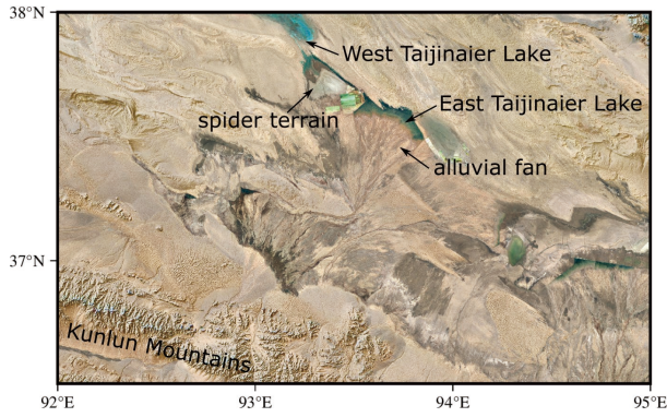
Fig. 3. The geographic background of the spider terrain in the Qaidam Basin (Google satellite images taken on November 28, 2012).
