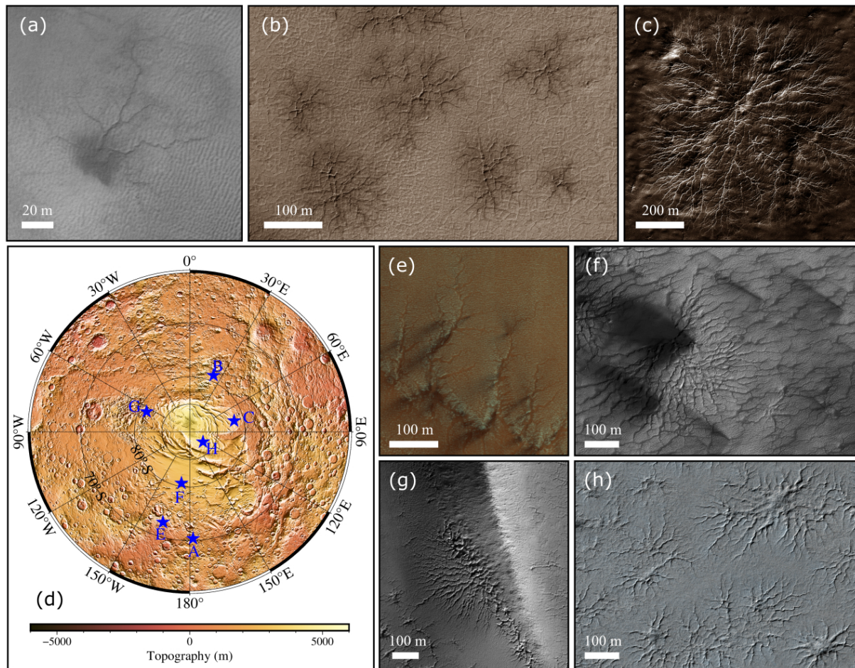
Fig. 1. Various araneiform morphologies were observed in the south polar region of Mars. (a) The early stage of the araneiform (ESP_023600_1095). (b) The middlescence stage of the araneiform (ESP_066587_0790). (c) The mature stage of the Martian araneiform with a good fractal structure (ESP_014255_0980). (d) The shaded relief map of the south polar region of Mars. The blue stars represent the locations of the corresponding araneiforms. (e) Parallel araneiforms that developed along a ditch (ESP_056038_1070). (f) Araneiform networks with meandering and wide channels (ESP_029613_0995). (g) The half araneiform developed under a dune (PSP_006204_0985). (h) Fat araneiforms (ESP_066555_0870).
