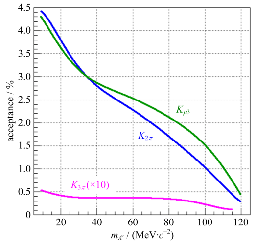
Fig. 7 Acceptances of the joint dark photon selection for K_{2\pi} , K_{\mu 3} and K_{3\pi} , depending on the assumed mass of the dark photon, evaluated with MC simulations
